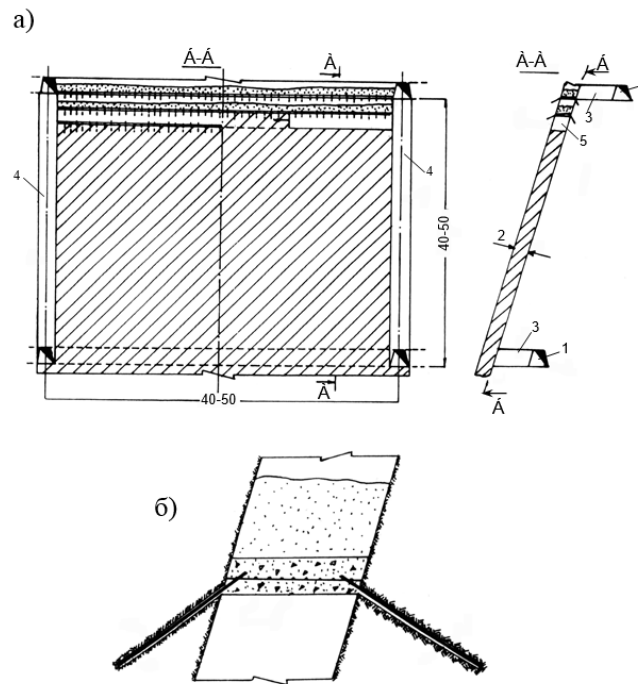
Figure 1. development system with descending top-slicing ore excavation (a) with interlayer overlap reinforced concrete enclosing (b)
