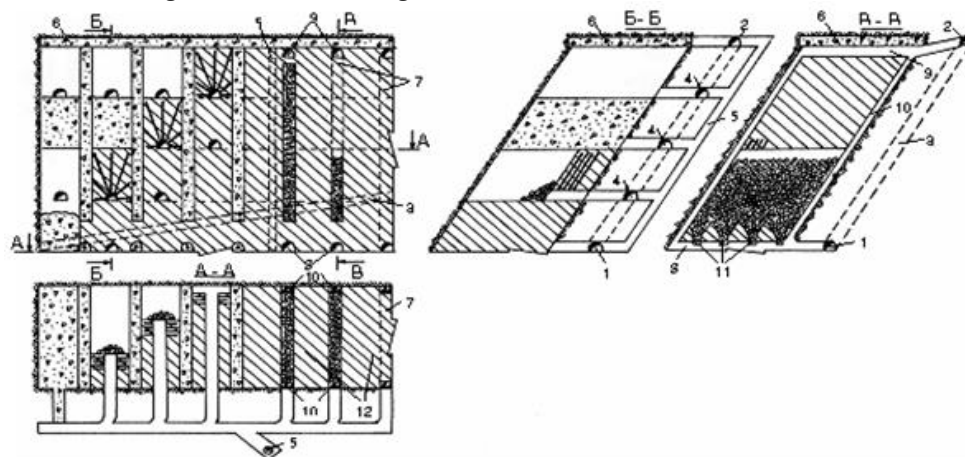
Figure 3. Combined development system with the formation of underground voids at the stable ore-rock mass
