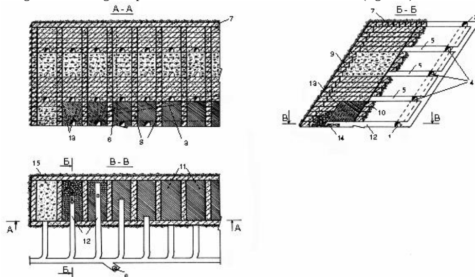
Figure 2. Combined development system with the formation of underground voids at unstable ore-rock mass
